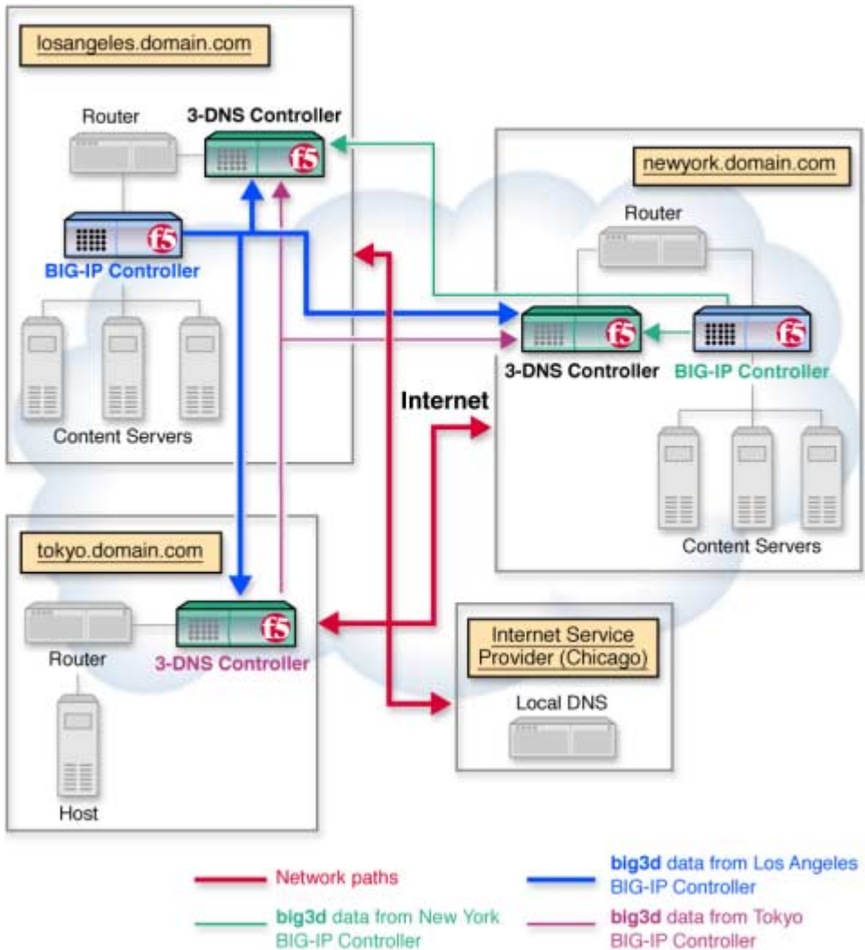
Figure 1.1 A sample network layout
