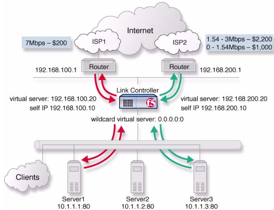
Figure 3.1 An example of cost-based ISP load balancing
