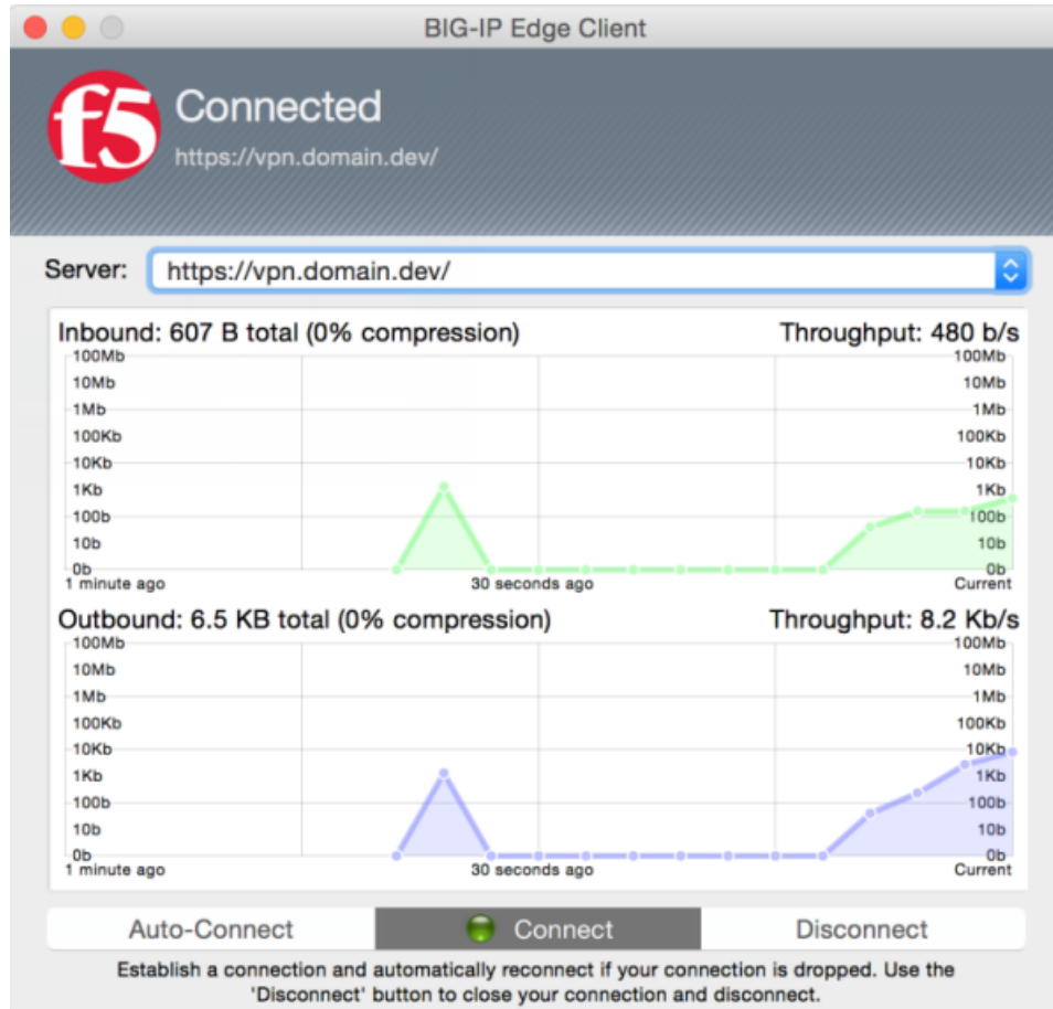
Figure 2: User interface on a Mac
