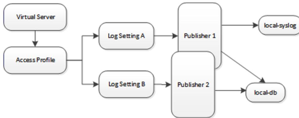
Figure 5: Event log duplication
