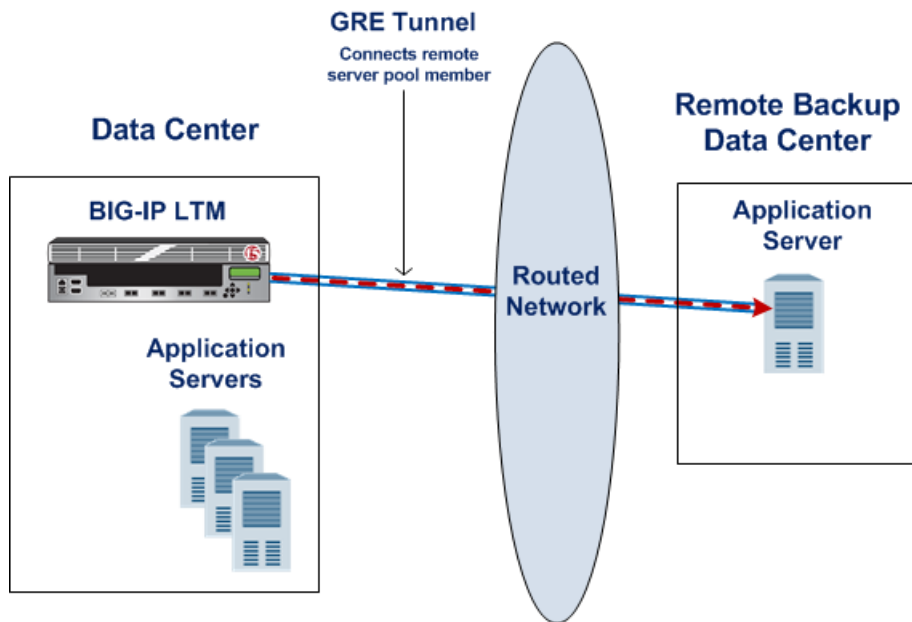
Figure 1: Illustration of a point-to-point GRE tunnel
