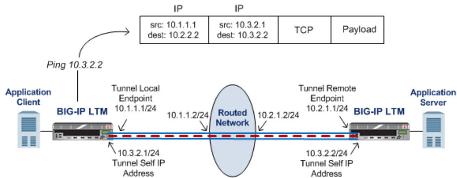
Figure 2: Illustration of a point-to-point IP tunnel configuration
