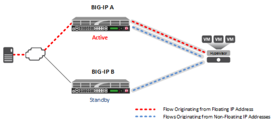
Figure 10: NVGRE tunnels configured for HA pair
