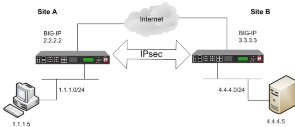
Figure 15: Example of an IPsec deployment
