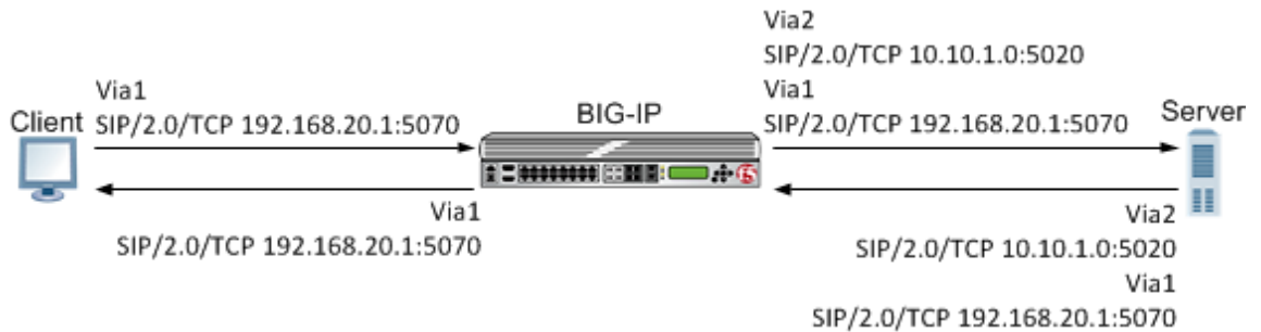
Figure 10: An example of SIP session traffic scenario 3
