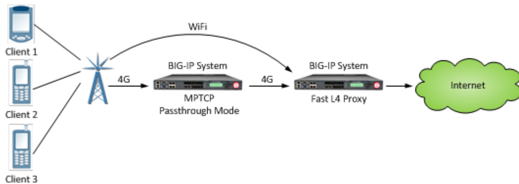
Figure 5: An MPTCP passthrough configuration
