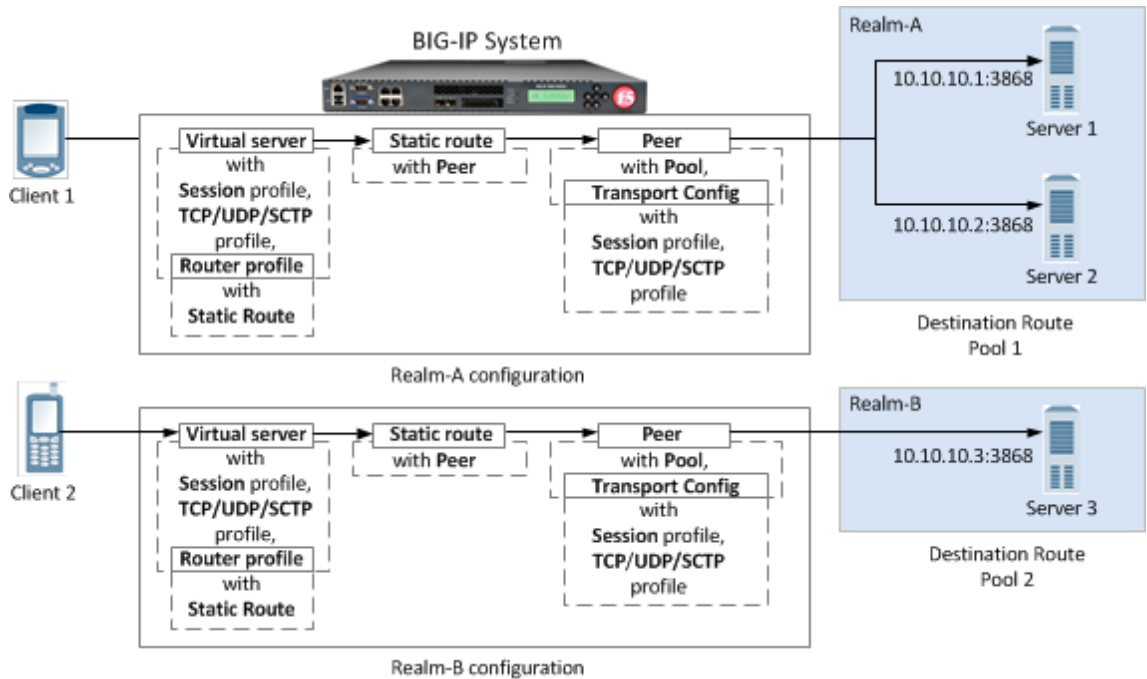
Figure 6: A Diameter message routing configuration
