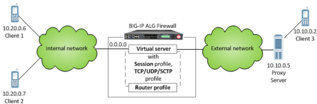
Figure 14: A SIP firewall configuration
