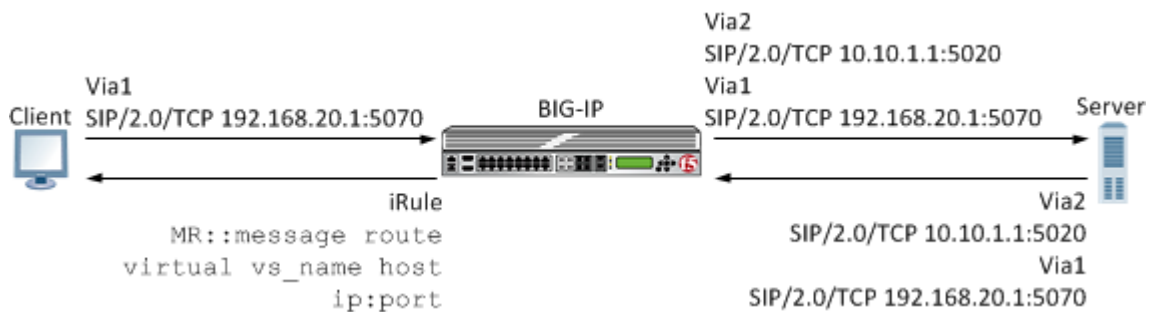
Figure 11: An example of SIP session traffic scenario 4
