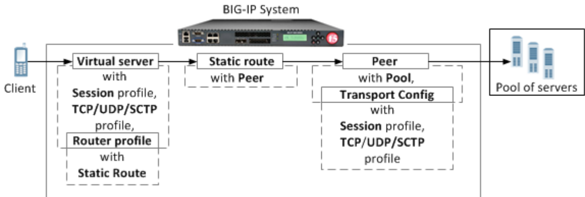
Figure 7: SIP proxy configuration objects
