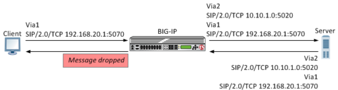
Figure 9: An example of SIP session traffic scenario 2
