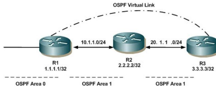
Figure 3: Multi-hop OSPFv3 Topology
