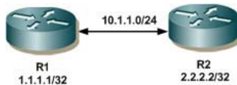
Figure 6: Basic Topology for BFD-ISIS
