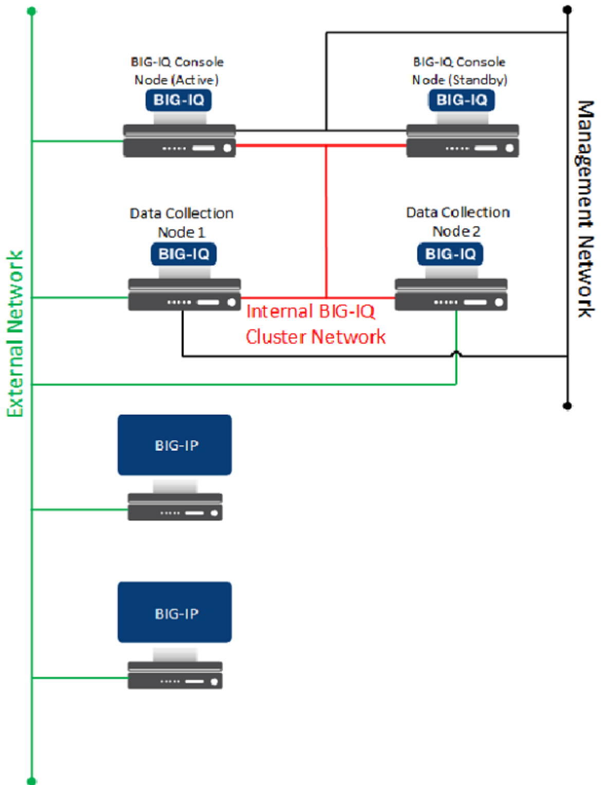
Figure 4: Centralized management, enhanced monitoring, and improved performance network topology
